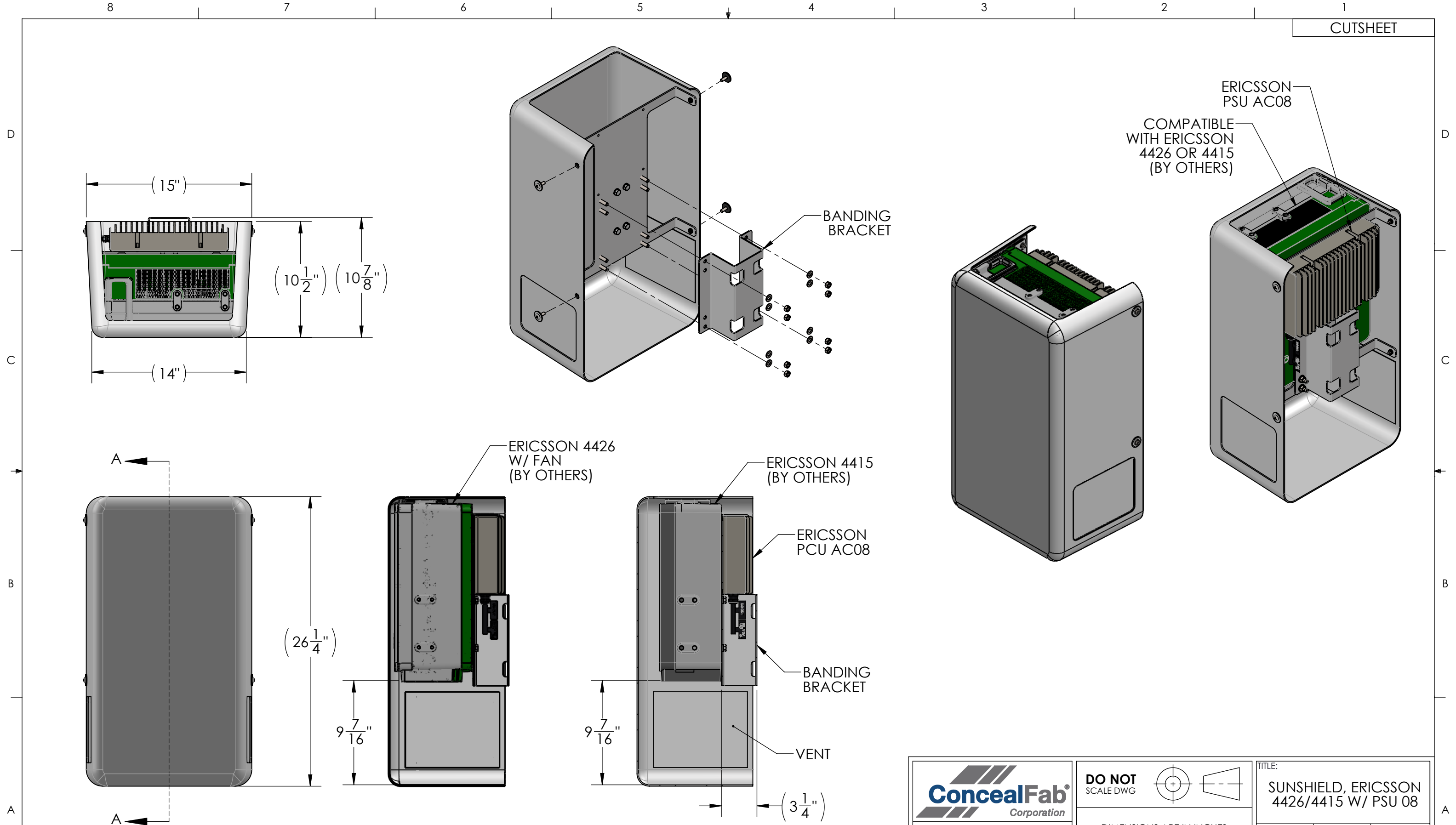
SECTION A-A (WITH ERICSSON 4426)
