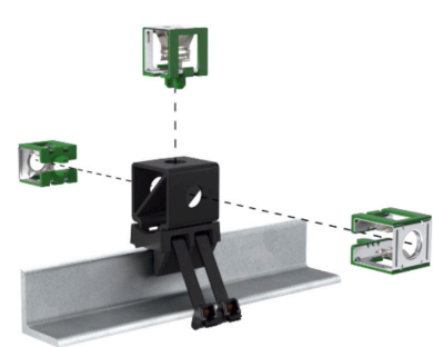
Universal Base with Snap-in Adapter 900713-10
