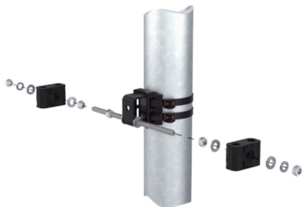
Threaded Rod Adapter with Universal Round Member base 900638-10
