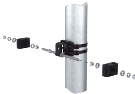
Universal Base with Threaded Rod Adapter 900712-10
