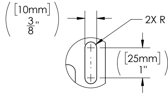
DETAIL B TYPICAL MOUNTING SLOT SCALE 1 : 2
